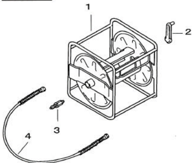
HR-55
